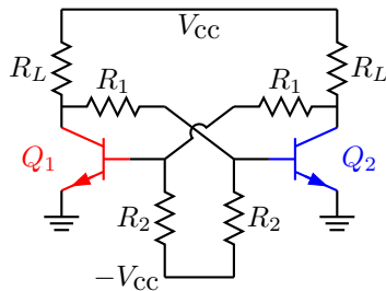
Figure 55: Bipolar transistor circuit, illustrating crossover and colored elements.
