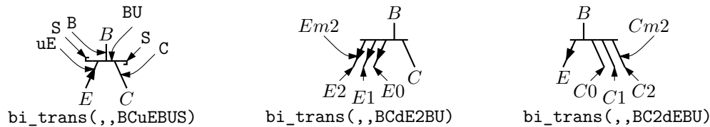
Figure 40: The bi_trans( linespec ,L|R, chars ,E) macro. The sub-elements are specified by the third argument. The substring E_n creates multiple emitters E_0 to E_n . Collectors are similar.
