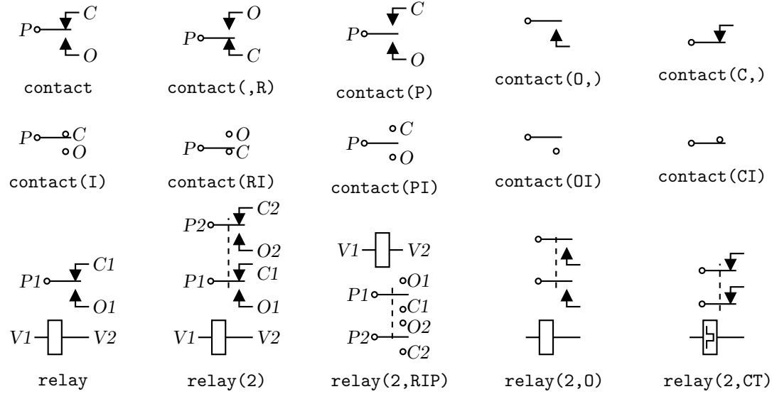
Figure 31: The contact(chars) and relay(poles, chars) macros (default direction right).
