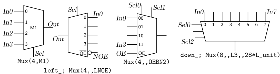
Figure 51: The Mux(input count, label, [L][B|H|X][N[n]|S[n]][[N]OE],wid,ht) macro.
