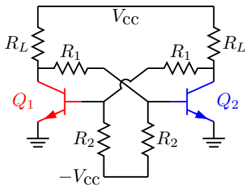
Figure 45: Bipolar transistor circuit, illustrating crossover and colored elements.
