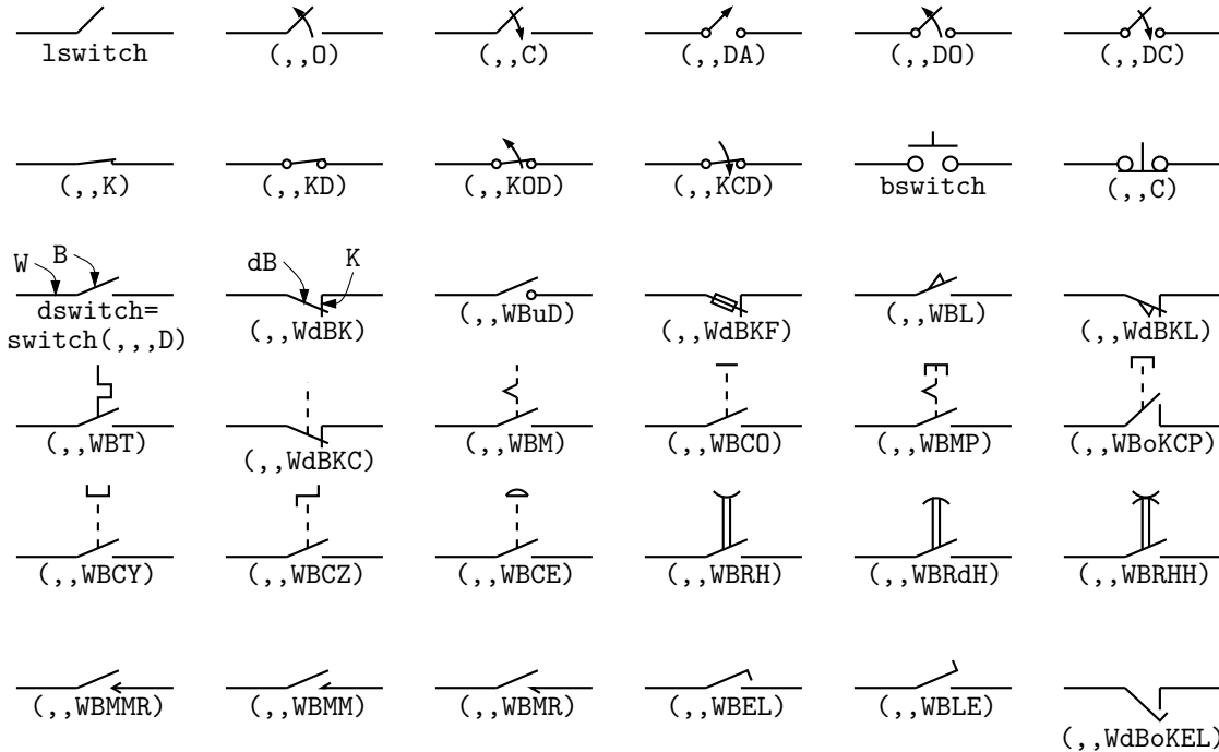
Figure 12: The switch( linespec , L | R , chars , L | B | D ) macro is a wrapper for the macros lswitch( linespec , [ L | R ], [ O | C ] [ D ] [ K ] [ A ]) , bswitch( linespec , [ L | R ], [ O | C ]) , and the many-optioned dswitch( linespec , R , W [ ud ] B [ K ] chars ) shown. The switch is drawn in the current drawing direction. A second-argument R produces a mirror image with respect to the drawing direction.
