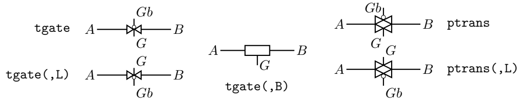
Figure 44: The tgate( linespec , [B] [R|L]) element, derived from a customized diode and ebox , and the ptrans( linespec , [R|L]) macro. These are not two-terminal elements, so the linespec argument defines the direction and length of the line from A to B but not the element position.
