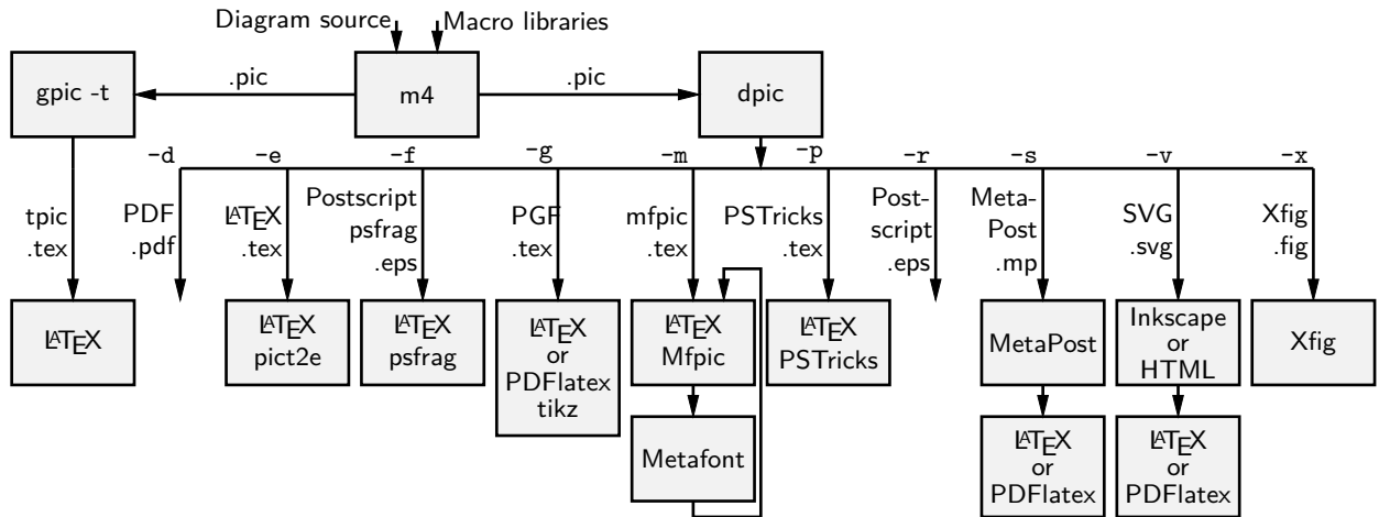
Figure 64: Output formats produced by gpict-t and dpic . SVG output can be read by Inkscape or used directly in web documents.
