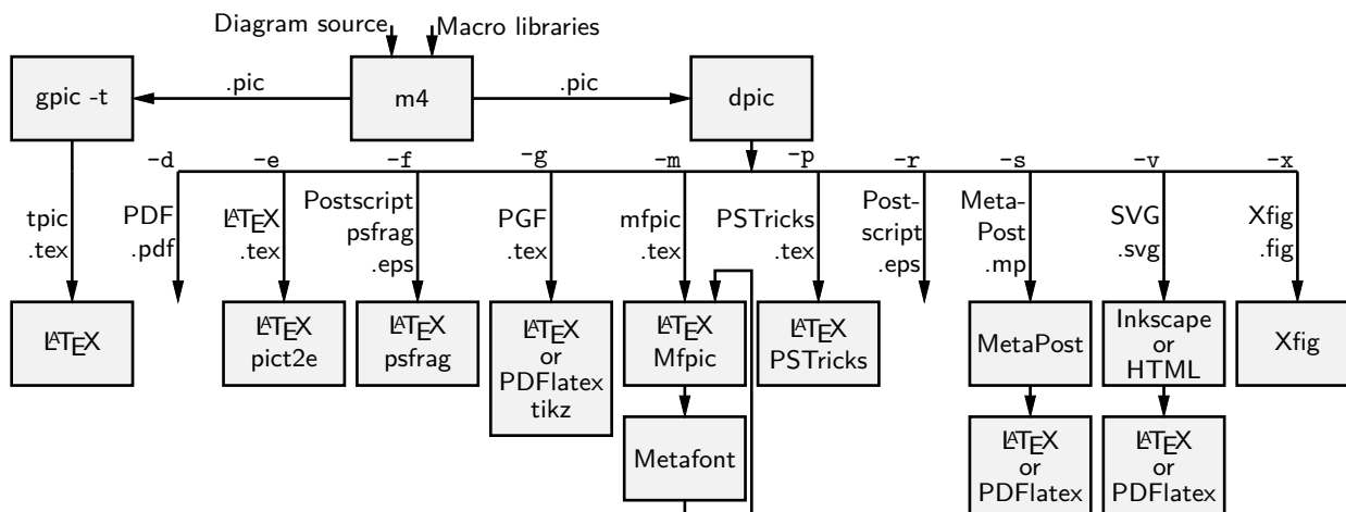
Figure 64: Output formats produced by gpic-t and dpic . SVG output can be read by Inkscape or used directly in web documents.
