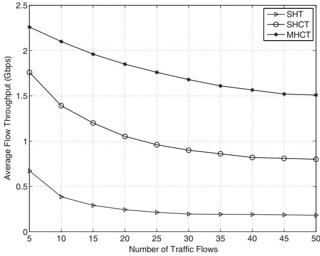
Fig. 8. Average flow throughput versus the number of traffic flows.
