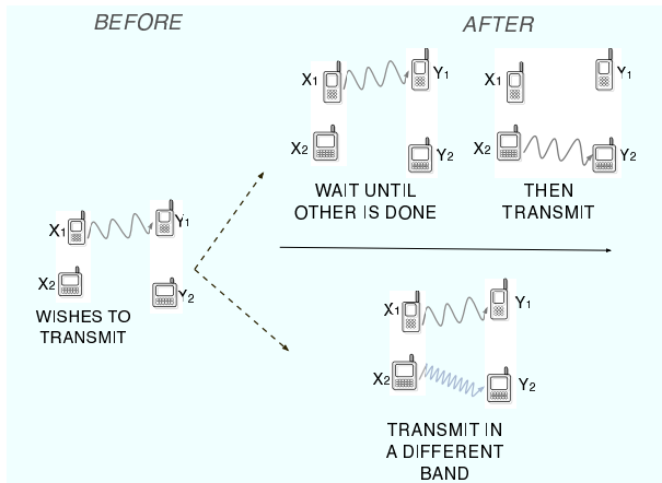
Fig. 1. Current proposals for dynamic spectrum leasing involve two schemes: when a cognitive radio X_2 wishes to transmit to Y_2 and a possibly non-cognitive X_1 is already transmitting to Y_1 , it can either wait until X_1 has completed its transmission (time division, as in the top figure), or possibly transmit at a different frequency band (frequency division, as in the bottom figure). In either case, time or frequency division is employed, rather than sharing the time/frequency spectrum.
