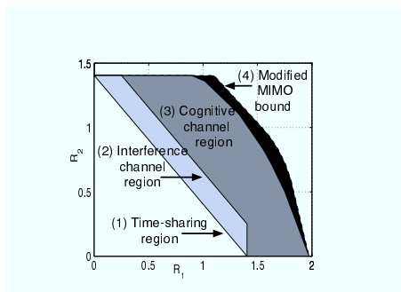
Fig. 3. Rate regions ( R_1, R_2 ) for different 2 sender, 2 receiver wireless channels. Region (1) is the time-sharing region of two independent senders. Region (2) is the best known achievable region for the interference channel, as calculated by Han and Kobayashi [9]. Region (3) is the achievable region described here and in [5] for the cognitive radio channel. Region (4) is an outer bound on the cognitive radio channel capacity. All simulations are in AWGN, with sender powers 6, and noise powers 1. The cross-over parameters in the interference channel are 0.55 and 0.55.
