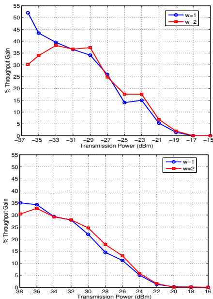
Fig. 10. Throughput gain of the JRM-BiNC-RA design with respect to the JRM-RA design: Top: Grid16; Bottom: Rand16 (averaged over 5 realizations).
