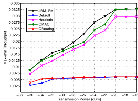
Fig. 5. Node throughput in the Rand16 network without network coding with w = 2 for different designs.
