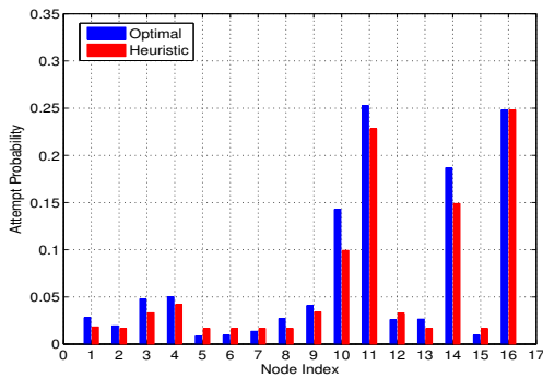
Fig. 8. Optimal and heuristic attempt probabilities in the Rand16 network at w = 1 , P_t = -34 dBm.
