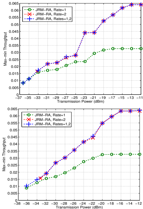
Fig. 6. Comparison of per node throughput between single rate and multi-rate cases with w = 2 : Top: Grid16; Bottom: Rand16.
