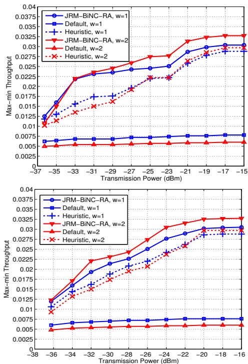
Fig. 9. Per node throughput in the two 16-node networks with network coding: Top: Grid16; Bottom: Rand16.
