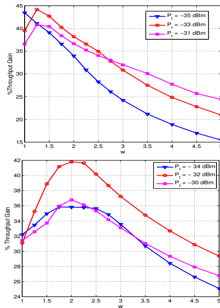
Fig. 11. Throughput gain versus w : Top: Grid16; Bottom: Rand16.
