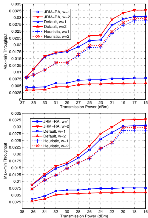
Fig. 4. Node throughput in the two 16-node networks without network coding: Top: Grid16; Bottom: Rand16.
