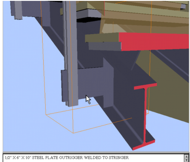
Figure 7. Experimental anchored notes in a VRML model.
