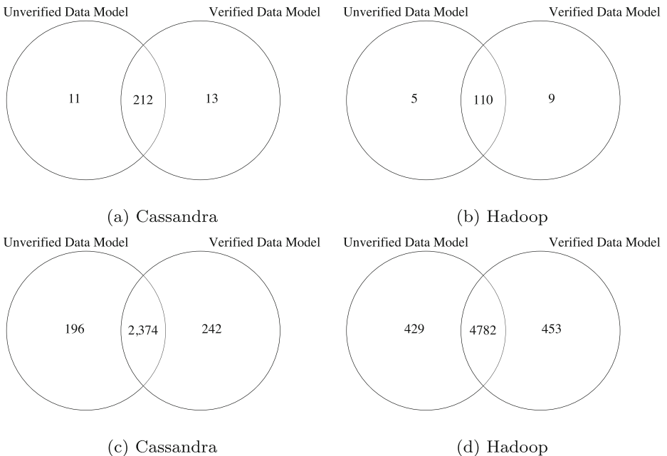
Fig. 7 Top: Comparison of correctly classified performance bug-inducing commits , before and after manual correction. Bottom: Comparison of correctly classified non-performance bug-inducing commits , before and after manual correction
