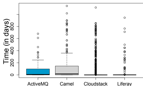
Fig. 5: Number of days before an added logging statement is changed in the studied applications
