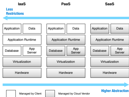
Figure 1: Basic models of cloud computing (following [8])
