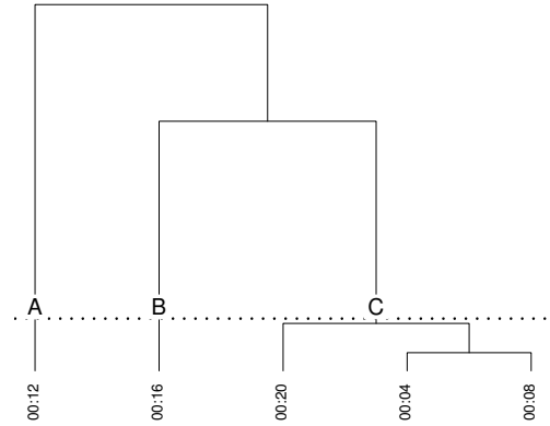
Fig. 2. Sample Dendrogram.
