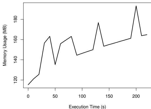
Fig. 3. Memory Usage
