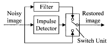
Fig. 1. A general framework of switching scheme-based image filters.
