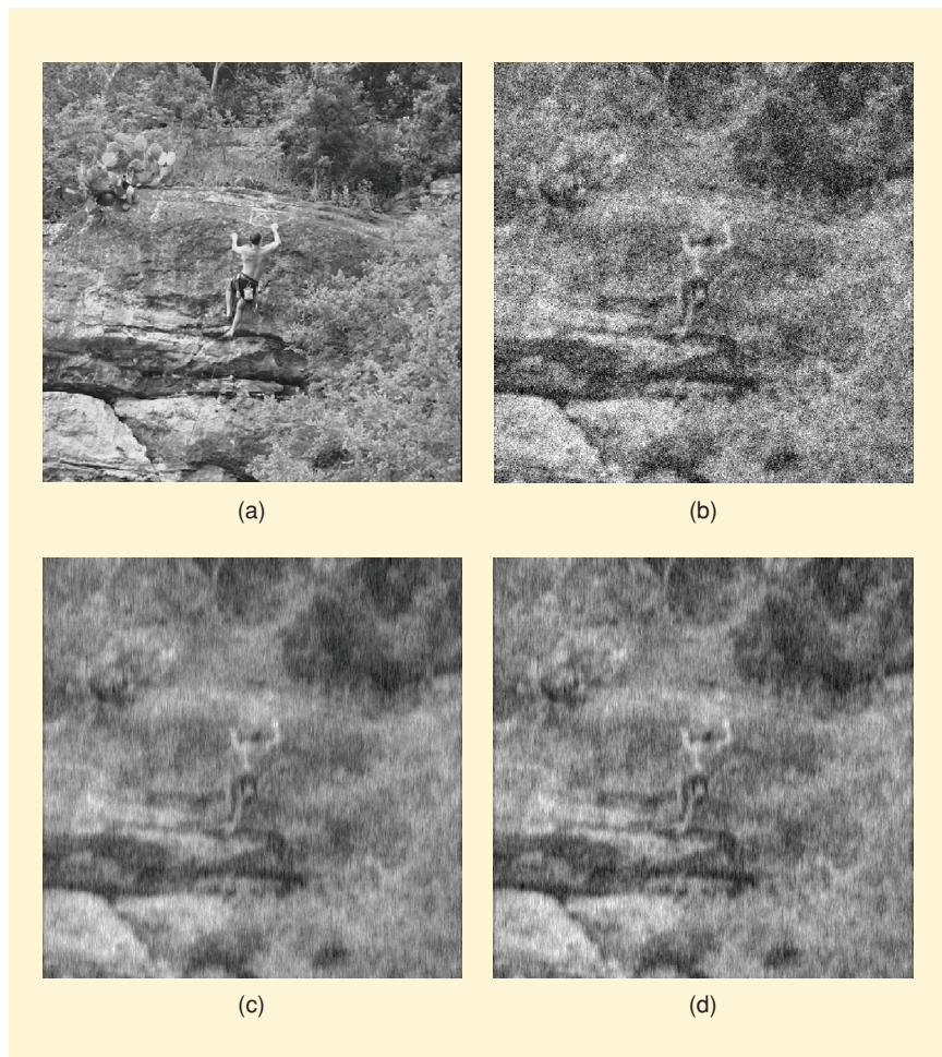
[FIG12] Linear image restoration. (a) Original image. (b) Blurred, noisy image (MSE = 3,131, SSIM = 0.27). (c) Image restored with linear MMSE filter (MSE = 1,064, SSIM = 0.35). (d) Restored using linear minimum stat-SSIM filter (MSE = 1,116, SSIM = 0.38).
