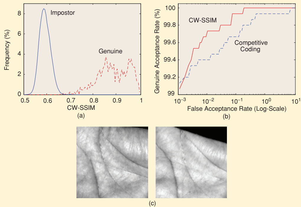
[FIG15] Palmpoint verification. (a) Genuine and impostor distributions of CW-SSIM. (b) ROC curves for CW-SSIM and competitive coding. (c) Two palmpoints from the same person that are correctly identified by CW-SSIM but not by the competitive coding algorithm.
