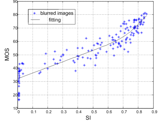
Fig. 3. Scatter plot of mean opinion score (MOS) versus SI model prediction of the blurred image dataset in LIVE database. Each data point represents one test image.
